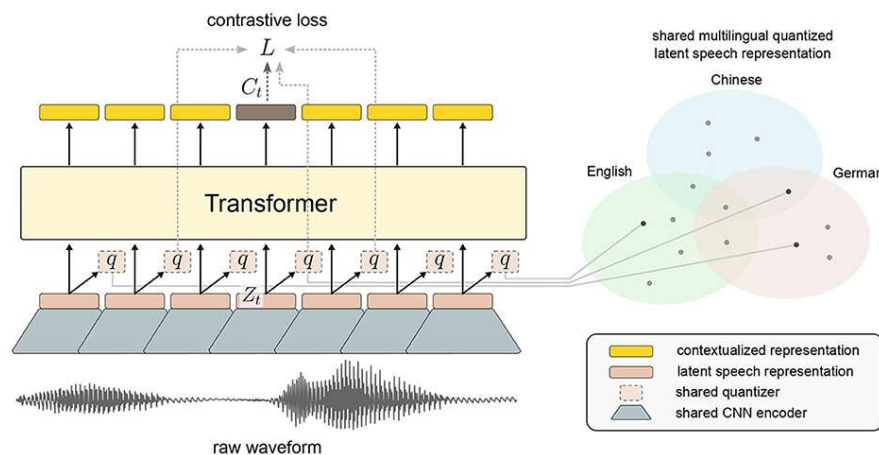
Figure 1. Framework of the wav2vec 2.0—XLSR pre-trained model.
