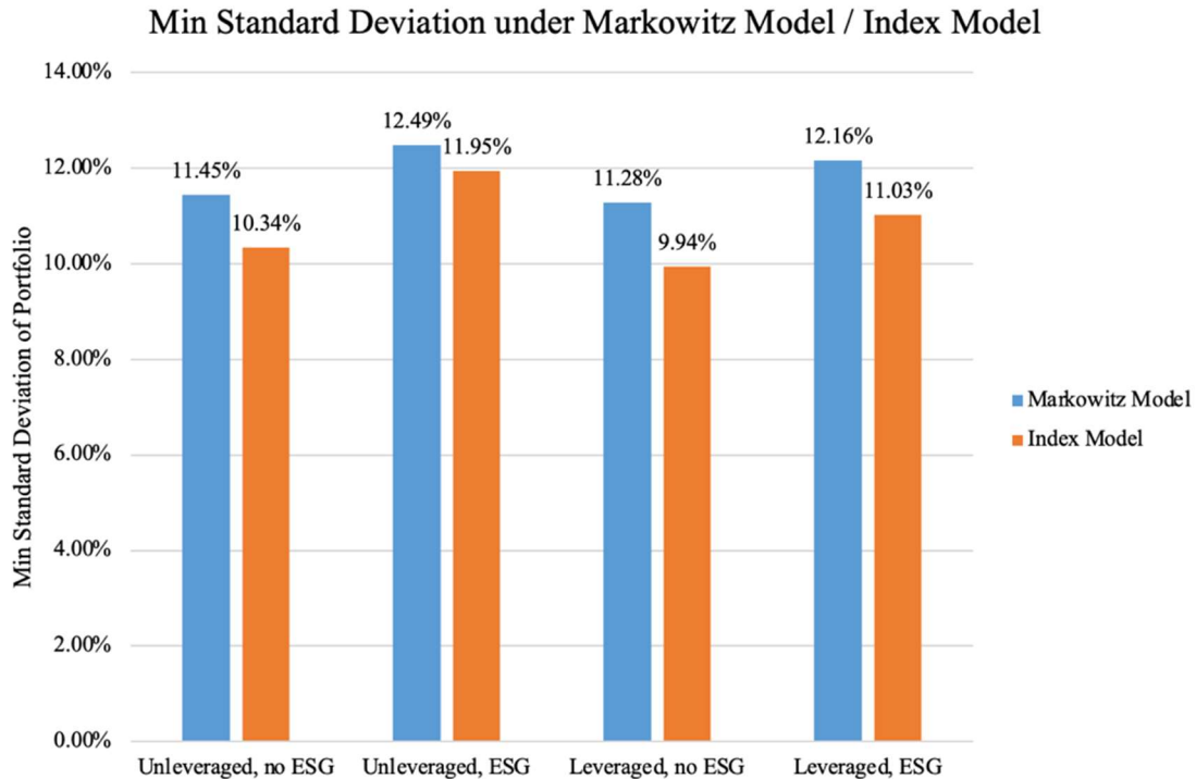
Figure 3. Min Standard Deviation under Markowitz Model / Index Model.
