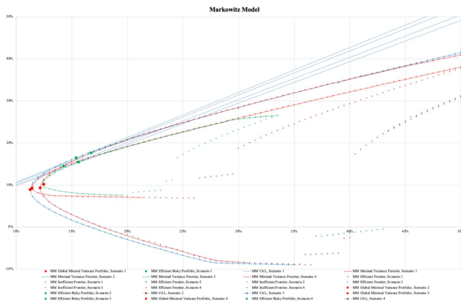
Figure 5. Efficient Frontier / Inefficient Frontier under the Markowitz Model.
