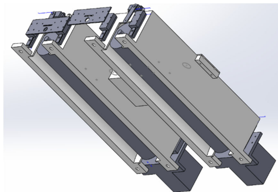
Figure 1. Overall structure of PV panel cleaning device
